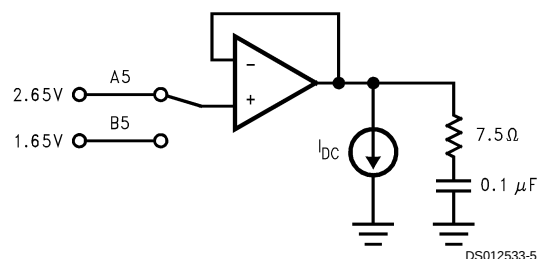
FIGURE 4. 13 mA Sink/Source
