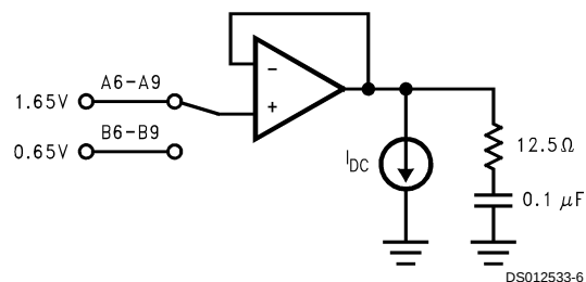
FIGURE 5. A6–A8: 13 mA Sink/Source A9: 13 mA Sink Only
